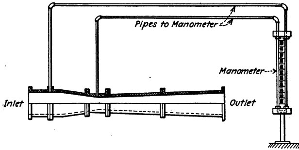
FIG. 135.—Venturi tube.
